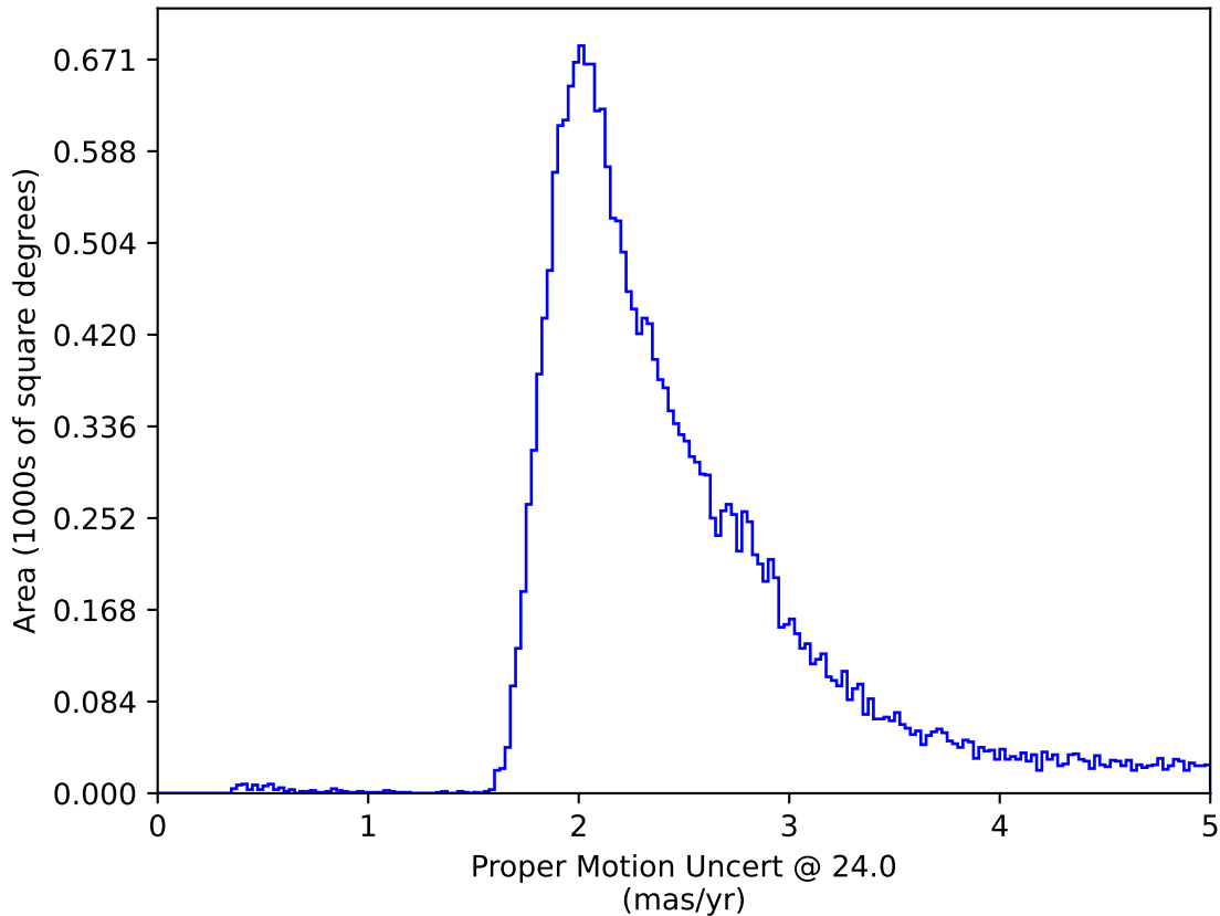
too_combined_s0.5_v3.4_10yrs All sky: Proper Motion Uncert @ 24.0
