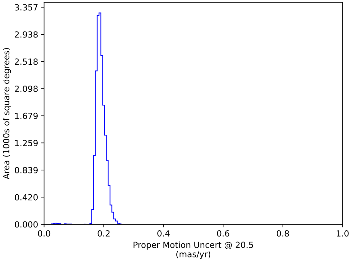
too_combined_s0.5_v3.4_10yrs WFD: Proper Motion Uncert @ 20.5
