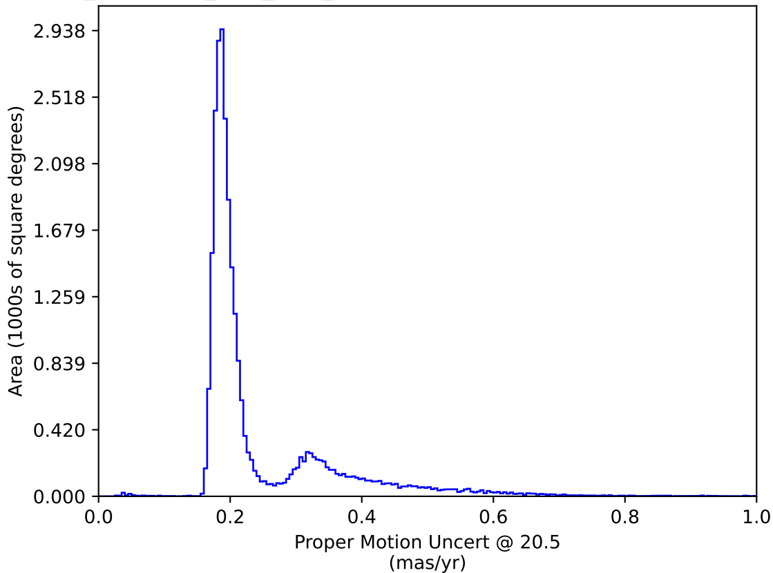
too_combined_s0.5_v3.4_10yrs All sky: Proper Motion Uncert @ 20.5
