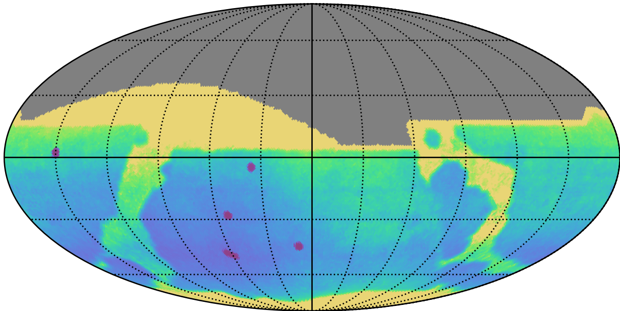
too_combined_s0.5_v3.4_10yrs All sky: Parallax Uncert @ 24.0
