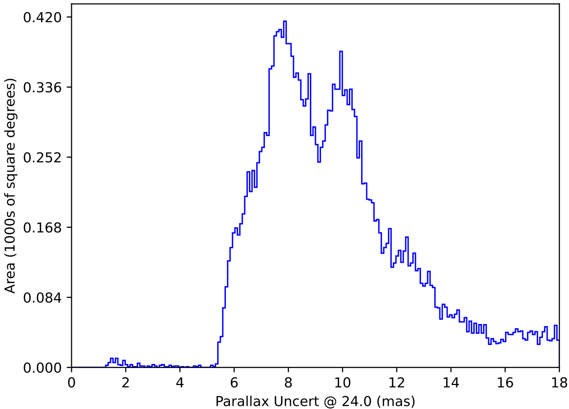
too_combined_s0.5_v3.4_10yrs All sky: Parallax Uncert @ 24.0
