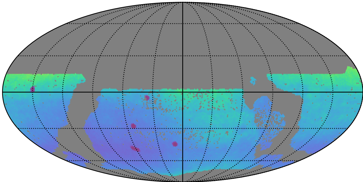
too_combined_s0.5_v3.4_10yrs WFD: Parallax Uncert @ 22.4
