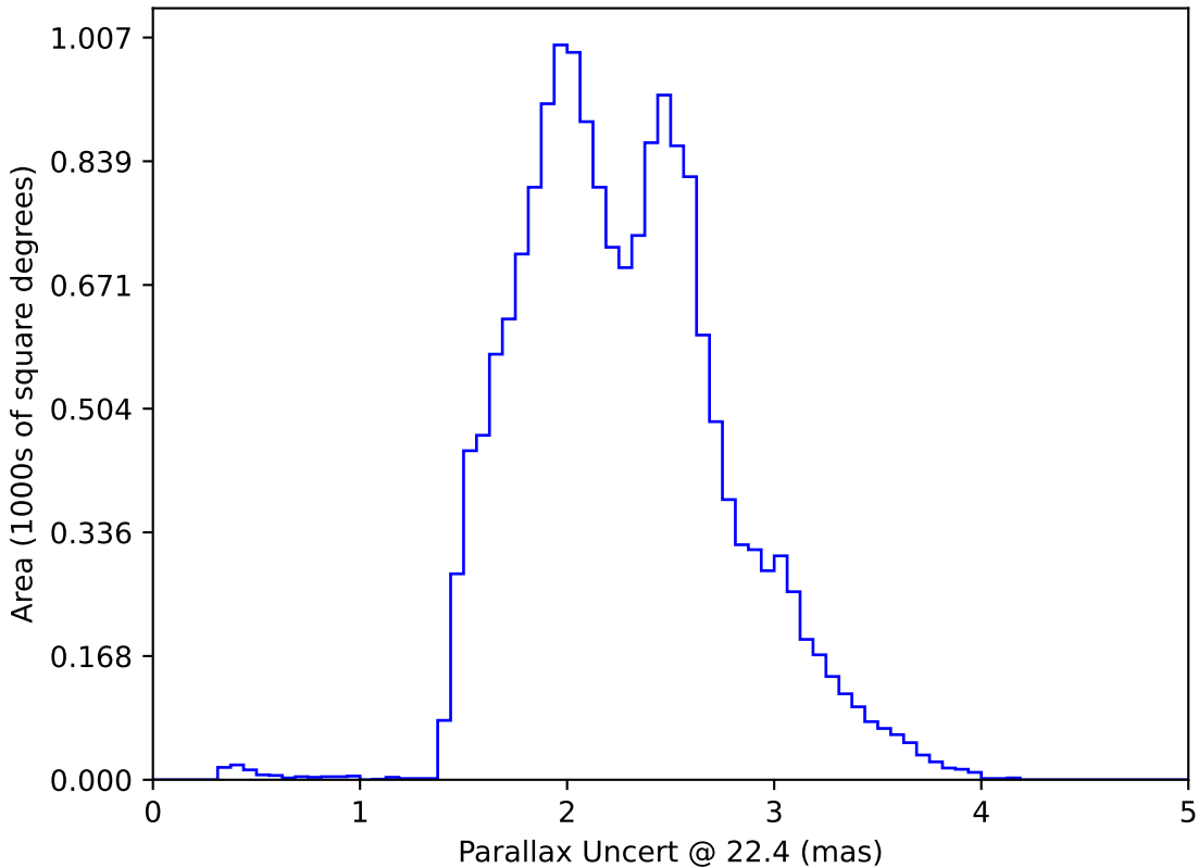
too_combined_s0.5_v3.4_10yrs WFD: Parallax Uncert @ 22.4
