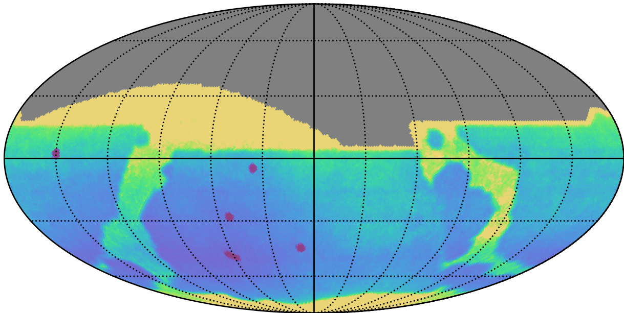
too_combined_s0.5_v3.4_10yrs All sky: Parallax Uncert @ 22.4
