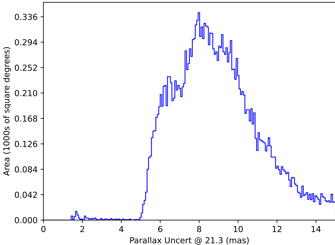
too_combined_s0.5_v3.4_10yrs All sky y band only: Parallax Uncert @ 21.3
