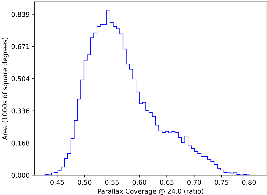
too_combined_s0.5_v3.4_10yrs WFD: Parallax Coverage @ 24.0
