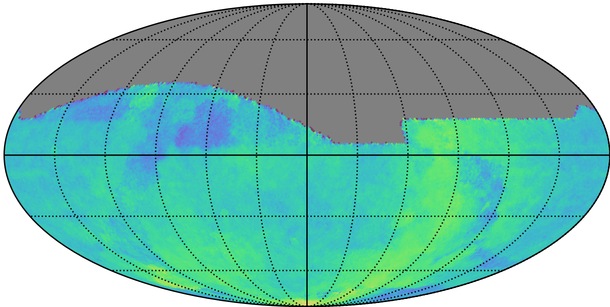
too_combined_s0.5_v3.4_10yrs All sky: Parallax Coverage @ 24.0
