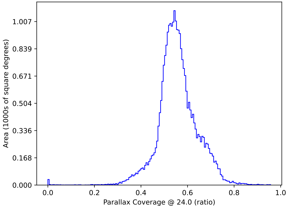
too_combined_s0.5_v3.4_10yrs All sky: Parallax Coverage @ 24.0
