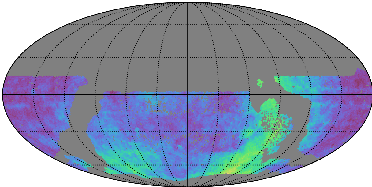
too_combined_s0.5_v3.4_10yrs WFD: Parallax Coverage @ 22.4
