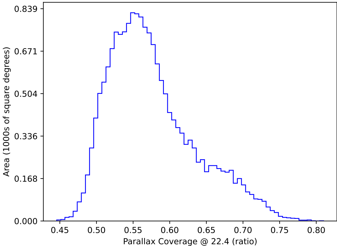
too_combined_s0.5_v3.4_10yrs WFD: Parallax Coverage @ 22.4
