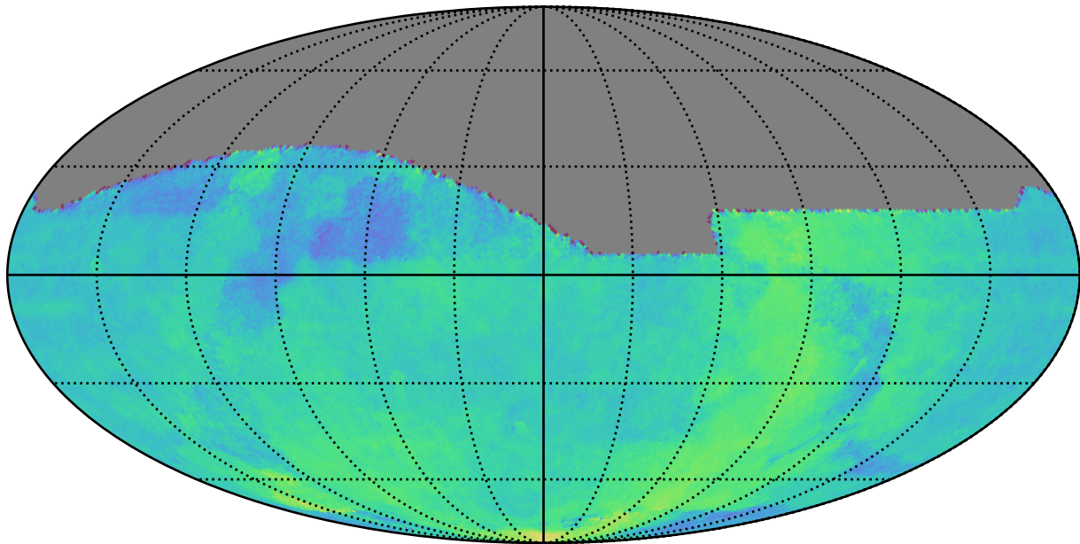
too_combined_s0.5_v3.4_10yrs All sky: Parallax Coverage @ 22.4
