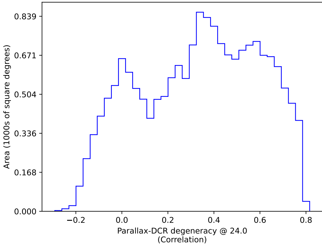
too_combined_s0.5_v3.4_10yrs WFD: Parallax-DCR degeneracy @ 24.0
