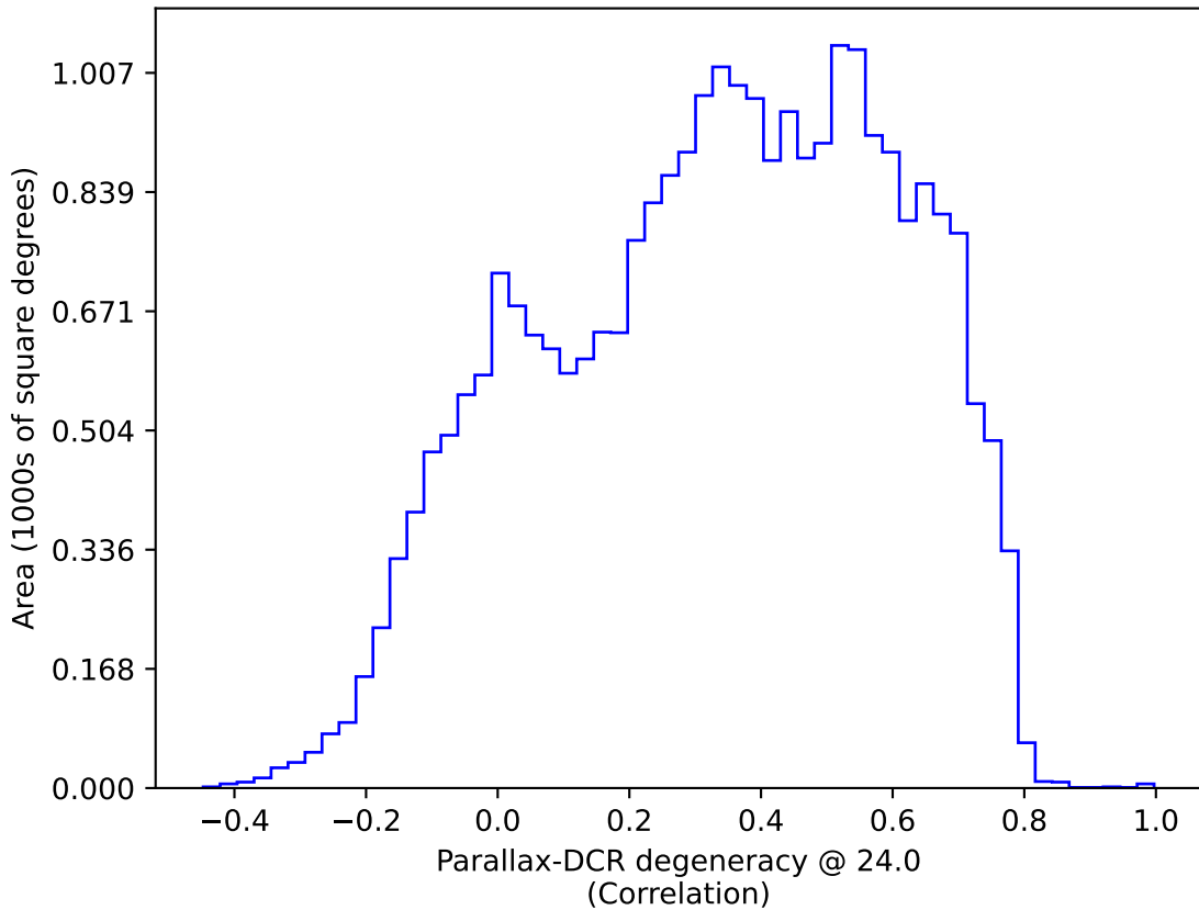
too_combined_s0.5_v3.4_10yrs All sky: Parallax-DCR degeneracy @ 24.0
