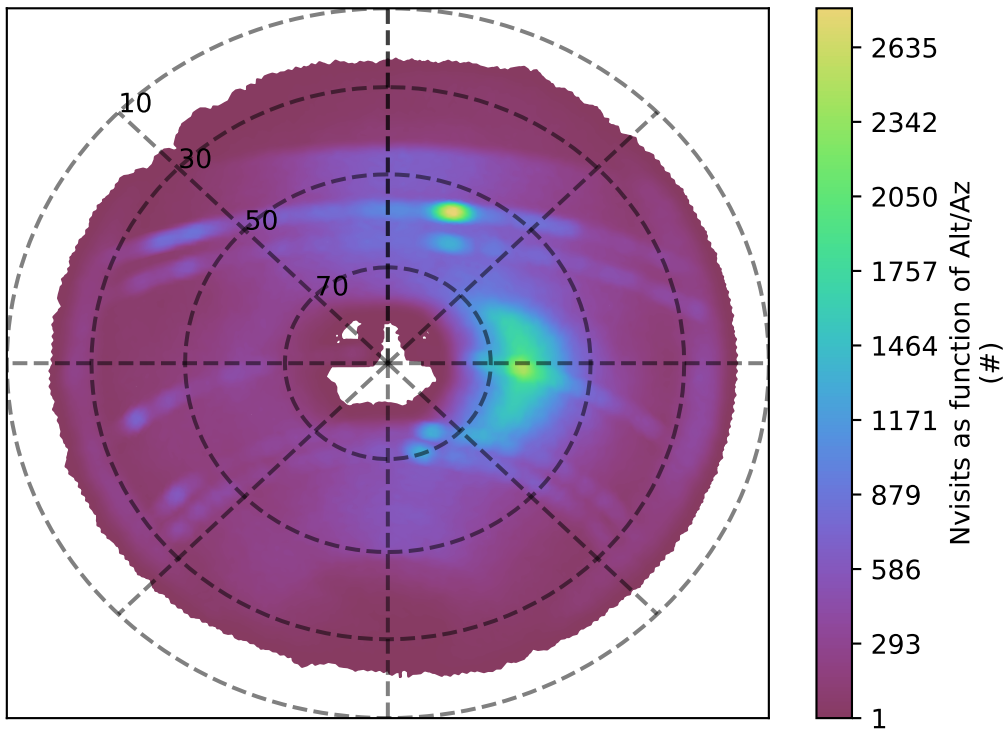
too_combined_s0.5_v3.4_10yrs z band: Nvisits as function of Alt/Az
