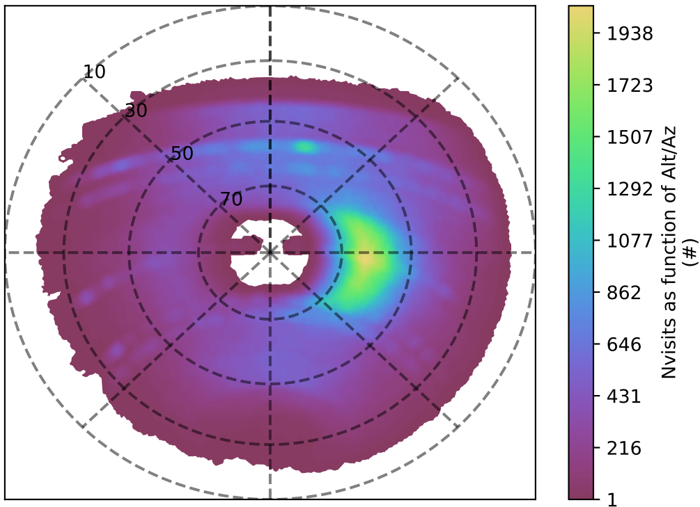
too_combined_s0.5_v3.4_10yrs y band: Nvisits as function of Alt/Az
