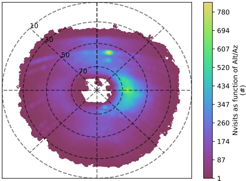
too_combined_s0.5_v3.4_10yrs u band: Nvisits as function of Alt/Az
