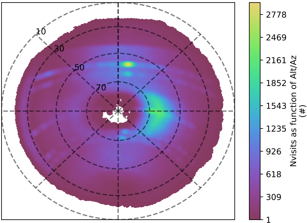
too_combined_s0.5_v3.4_10yrs r band: Nvisits as function of Alt/Az
