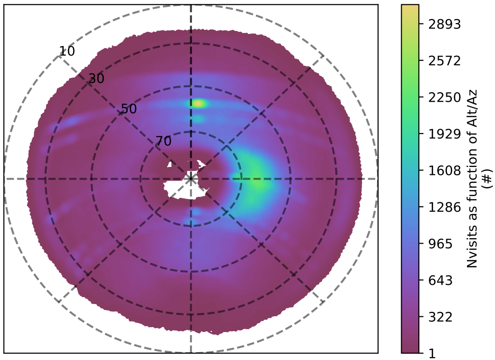
too_combined_s0.5_v3.4_10yrs i band: Nvisits as function of Alt/Az
