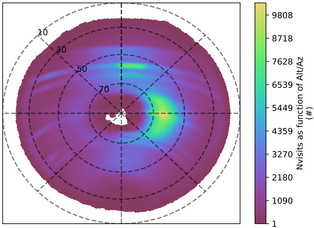
too_combined_s0.5_v3.4_10yrs all bands: Nvisits as function of Alt/Az
