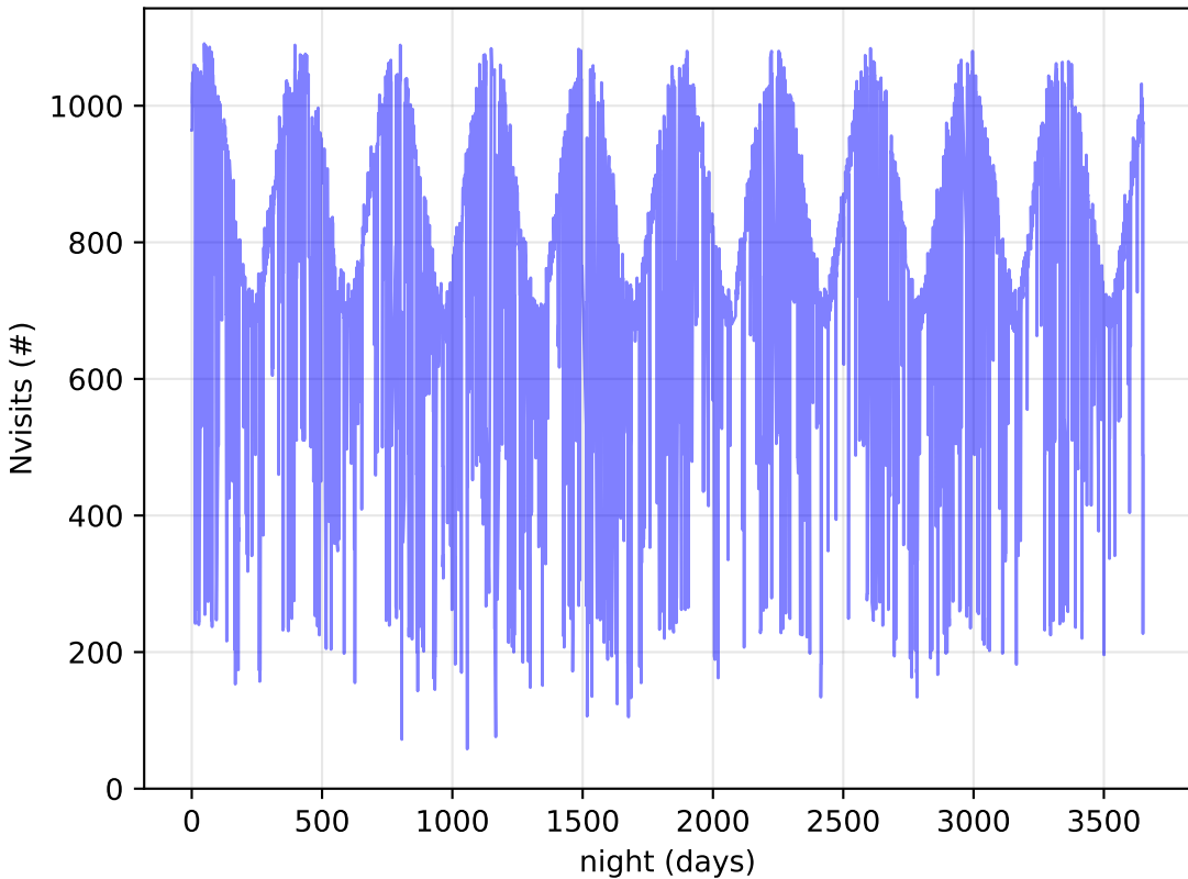
too_combined_s0.5_v3.4_10yrs All visits: Nvisits
