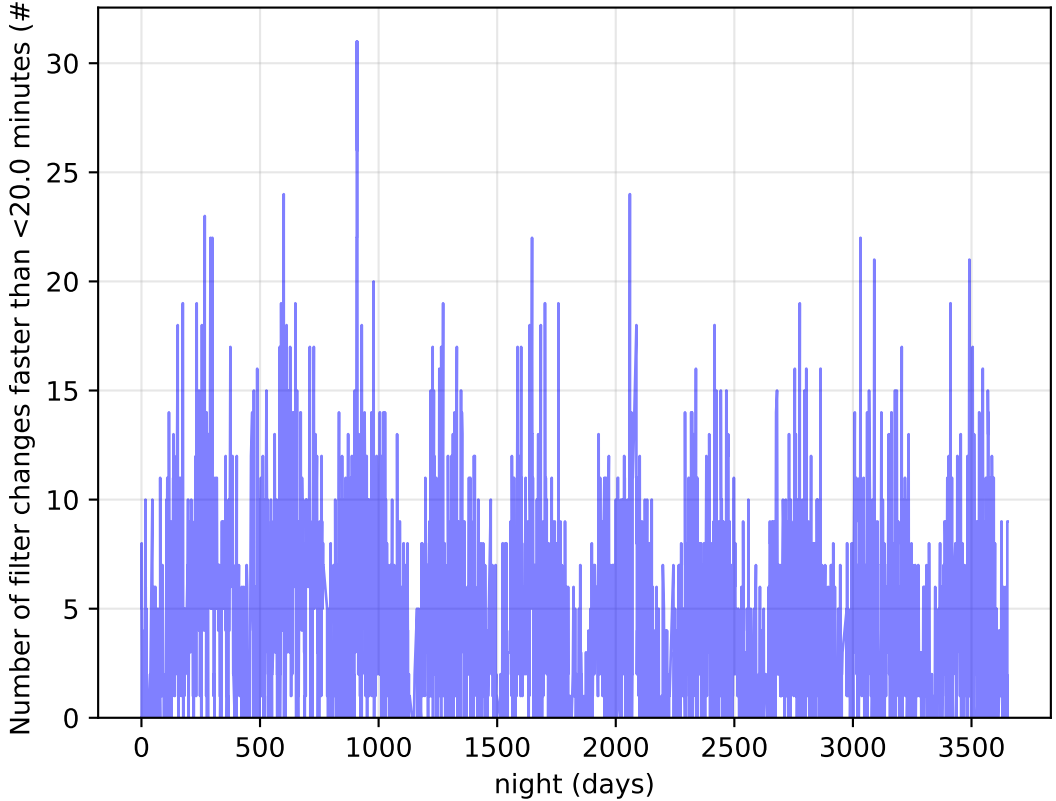
too_combined_s0.5_v3.4_10yrs Per Night: Number of filter changes faster than <20.0 minutes
