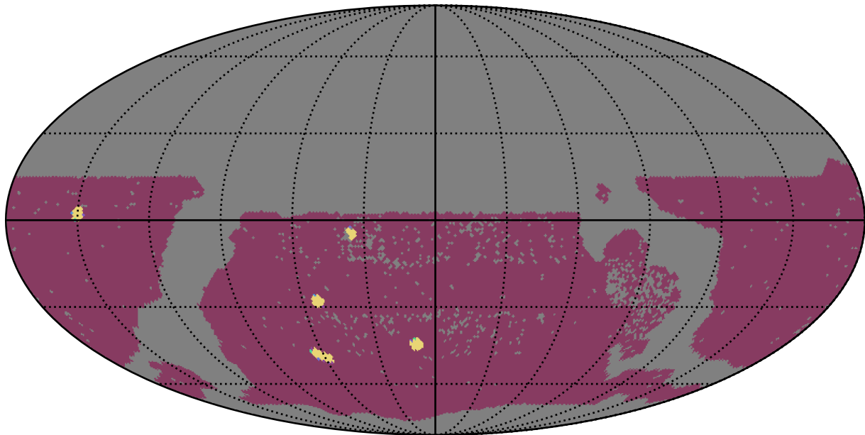
too_combined_s0.5_v3.4_10yrs WFD: NumberOfQuickRevisits
