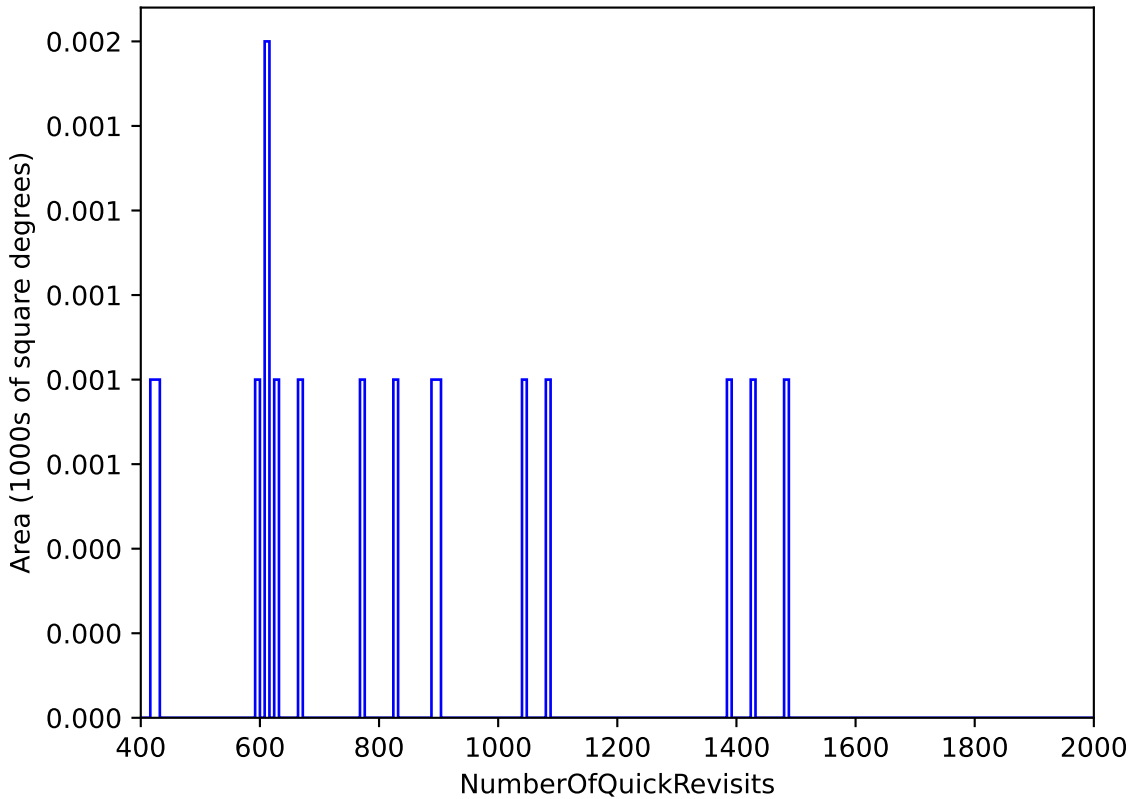
too_combined_s0.5_v3.4_10yrs WFD: NumberOfQuickRevisits
