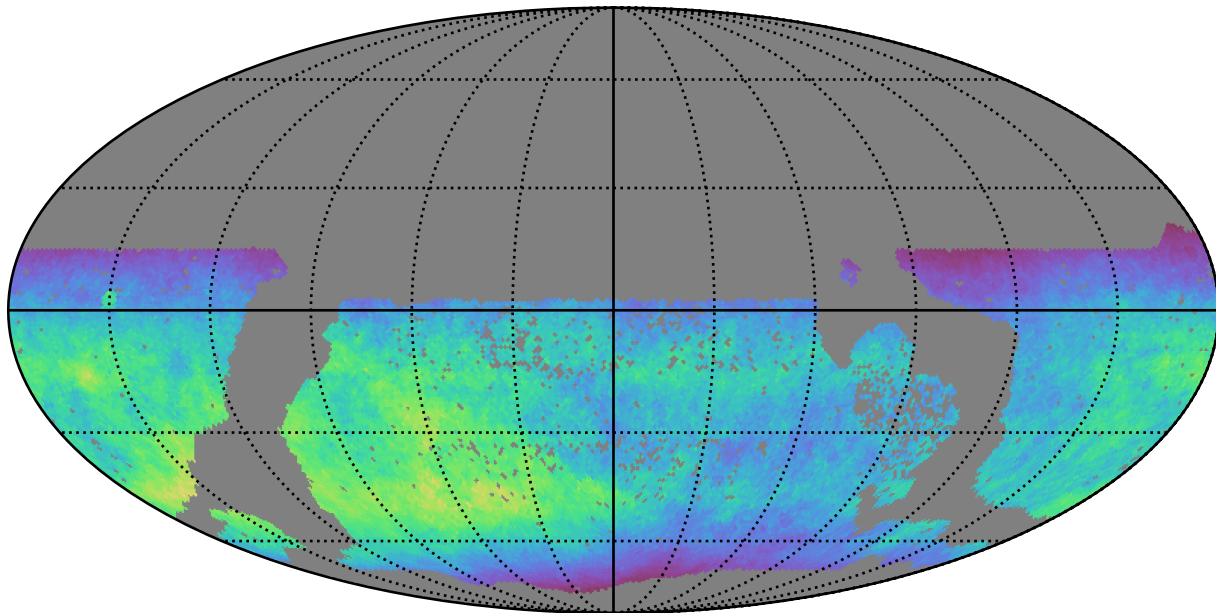
too_combined_s0.5_v3.4_10yrs WFD z band: Normalized Teff
