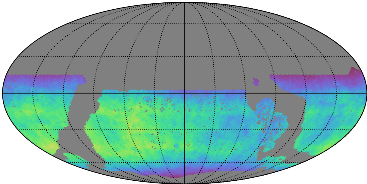
too_combined_s0.5_v3.4_10yrs WFD y band: Normalized Teff
