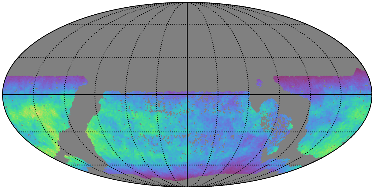
too_combined_s0.5_v3.4_10yrs WFD u band: Normalized Teff
