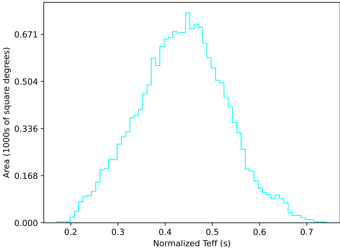
too_combined_s0.5_v3.4_10yrs WFD u band: Normalized Teff
