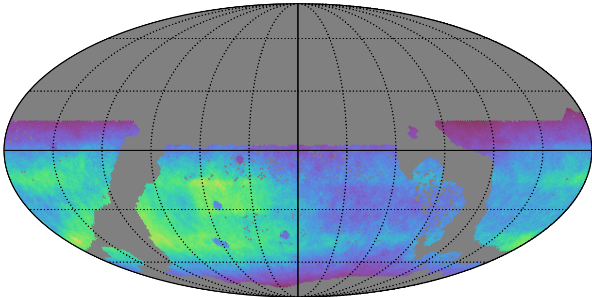
too_combined_s0.5_v3.4_10yrs WFD r band: Normalized Teff
