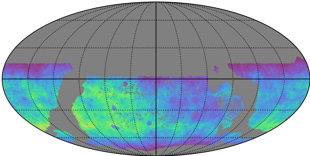
too_combined_s0.5_v3.4_10yrs WFD g band: Normalized Teff
