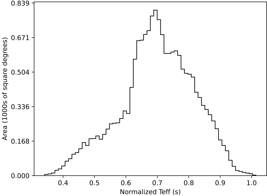
too_combined_s0.5_v3.4_10yrs WFD all bands: Normalized Teff
