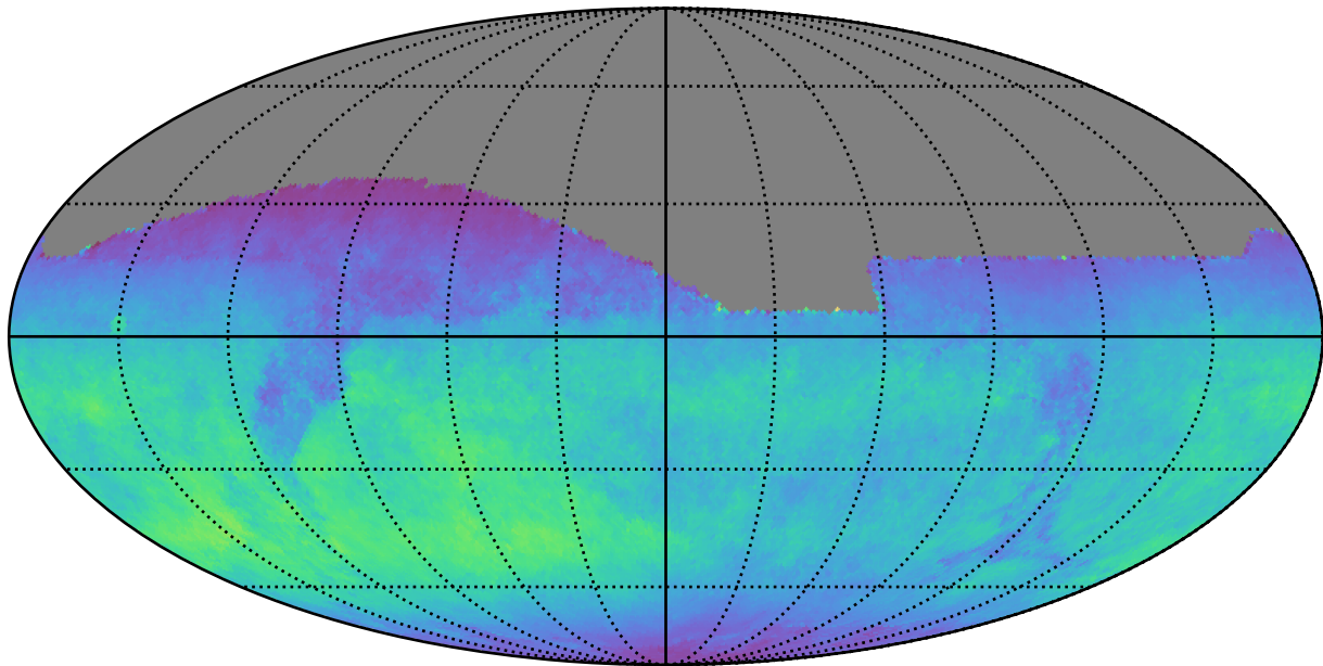
too_combined_s0.5_v3.4_10yrs All sky z band: Normalized Teff
