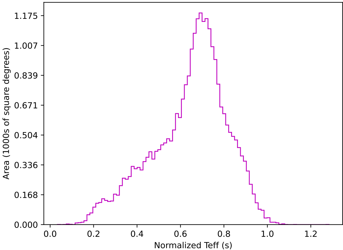
too_combined_s0.5_v3.4_10yrs All sky z band: Normalized Teff
