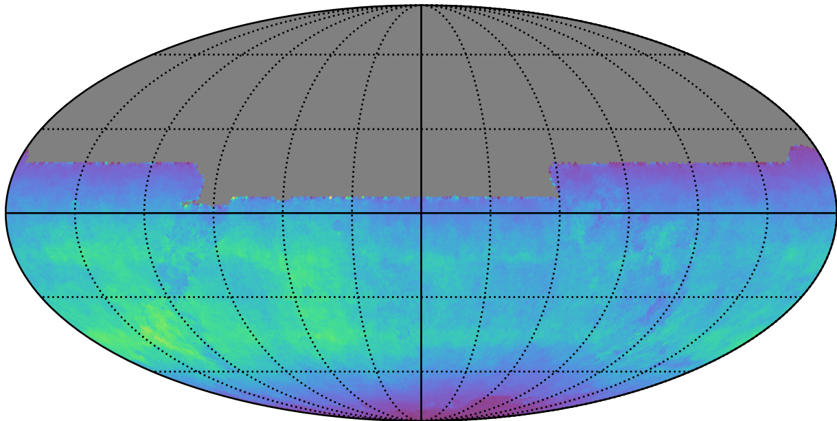
too_combined_s0.5_v3.4_10yrs All sky y band: Normalized Teff
