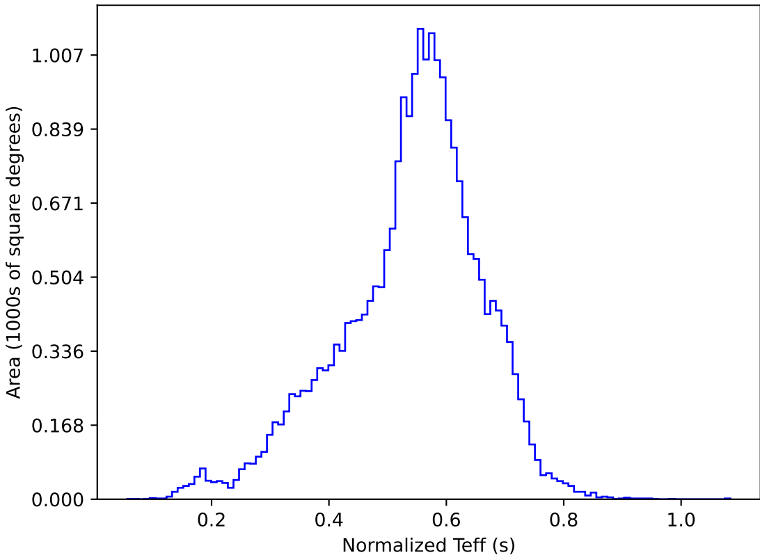
too_combined_s0.5_v3.4_10yrs All sky y band: Normalized Teff
