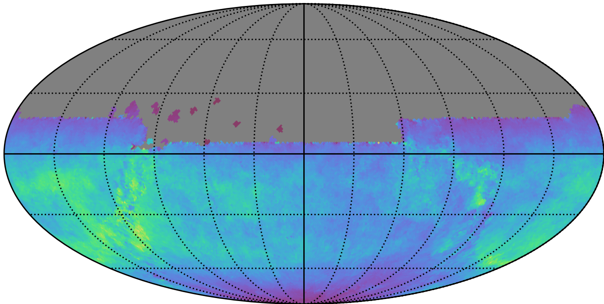
too_combined_s0.5_v3.4_10yrs All sky u band: Normalized Teff
