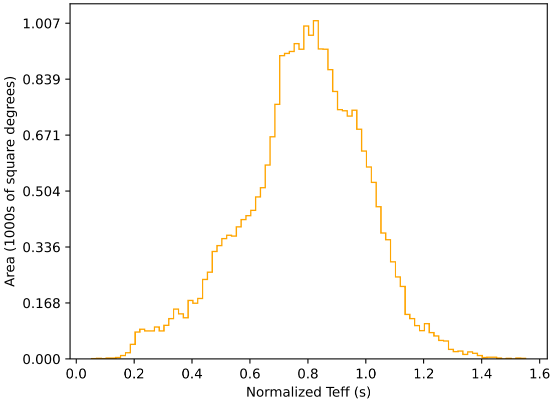
too_combined_s0.5_v3.4_10yrs All sky r band: Normalized Teff
