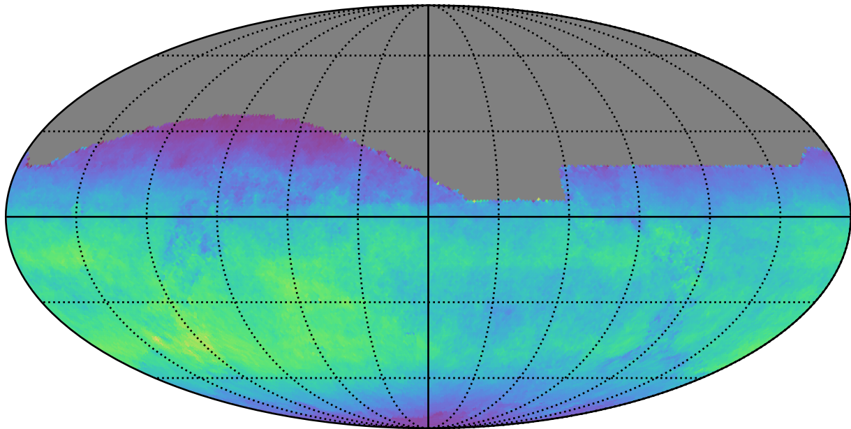
too_combined_s0.5_v3.4_10yrs All sky i band: Normalized Teff
