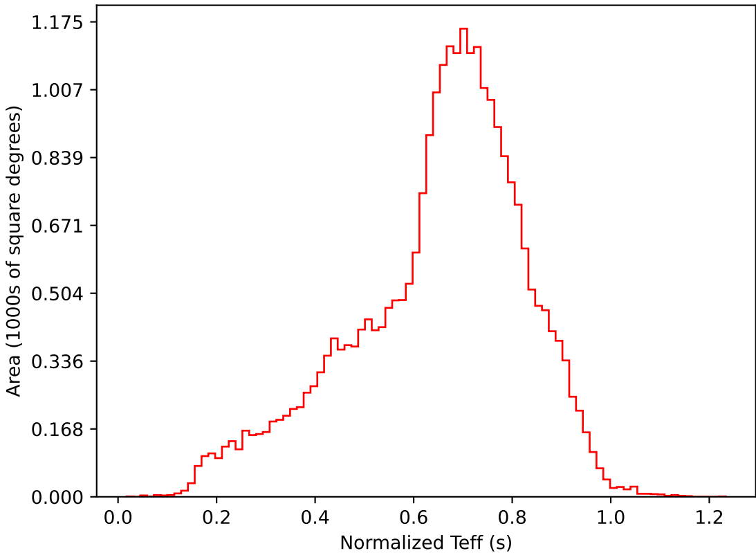
too_combined_s0.5_v3.4_10yrs All sky i band: Normalized Teff
