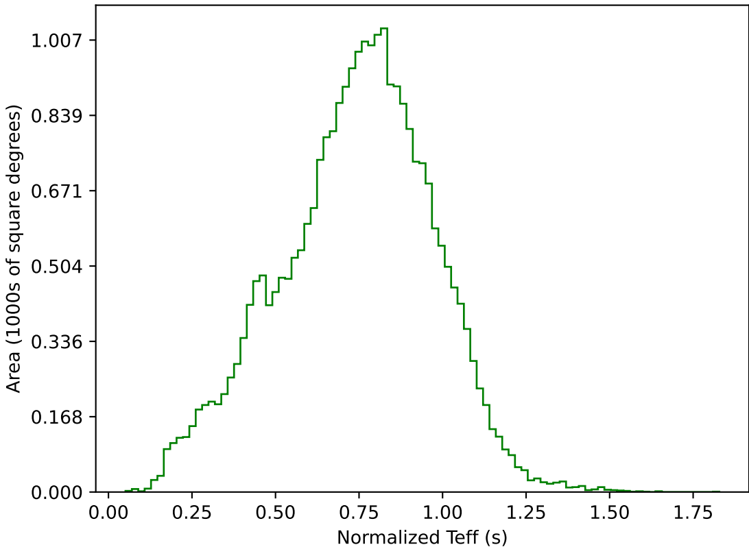
too_combined_s0.5_v3.4_10yrs All sky g band: Normalized Teff
