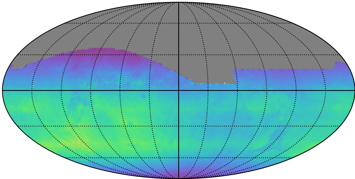
too_combined_s0.5_v3.4_10yrs All sky all bands: Normalized Teff
