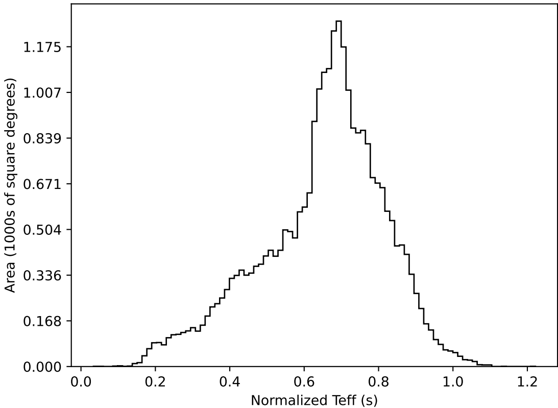
too_combined_s0.5_v3.4_10yrs All sky all bands: Normalized Teff
