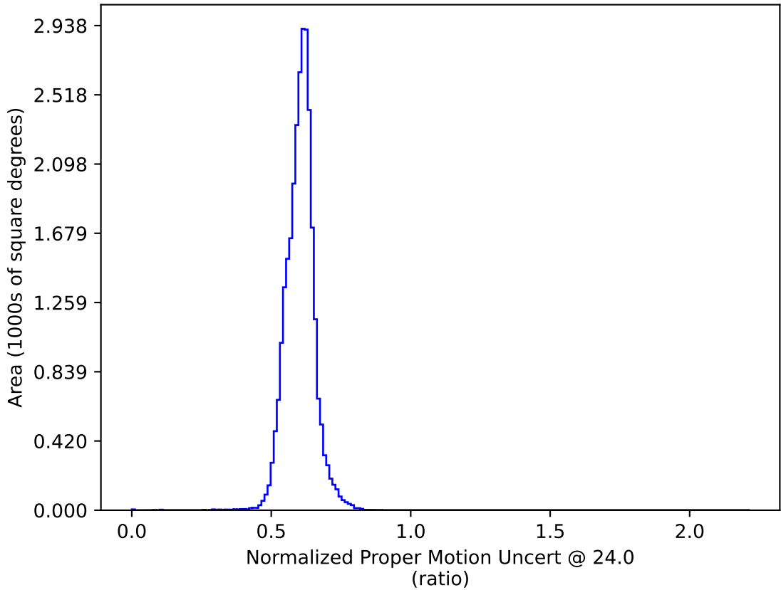
too_combined_s0.5_v3.4_10yrs All sky: Normalized Proper Motion Uncert @ 24.0
