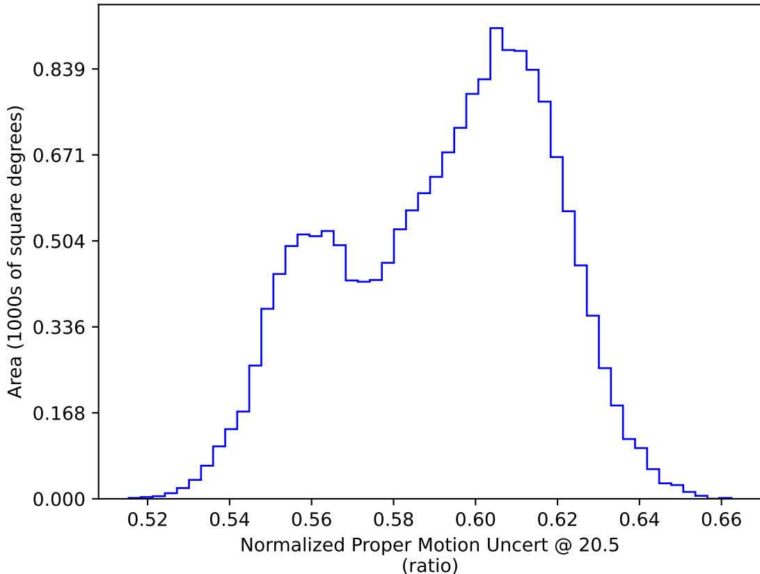
too_combined_s0.5_v3.4_10yrs WFD: Normalized Proper Motion Uncert @ 20.5
