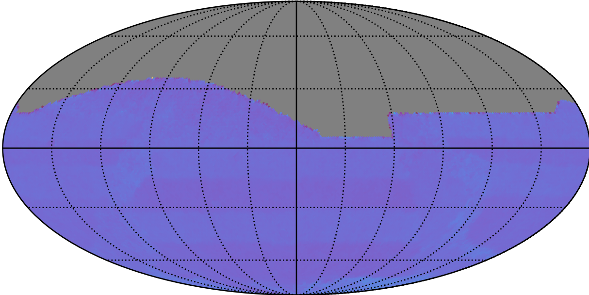
too_combined_s0.5_v3.4_10yrs All sky: Normalized Proper Motion Uncert @ 20.5
