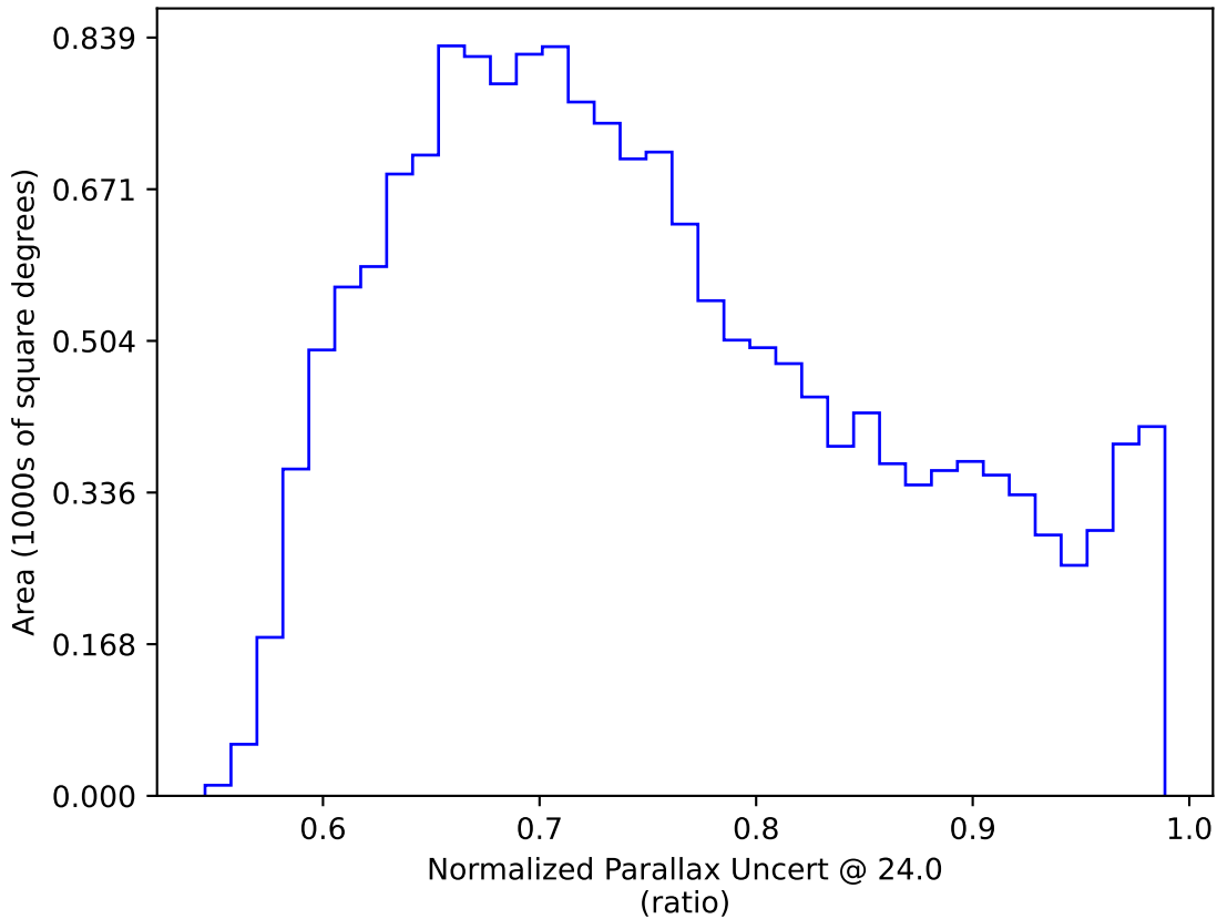
too_combined_s0.5_v3.4_10yrs WFD: Normalized Parallax Uncert @ 24.0
