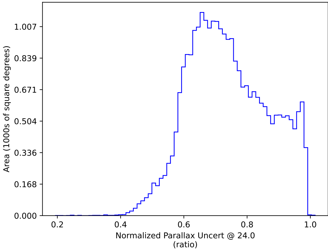
too_combined_s0.5_v3.4_10yrs All sky: Normalized Parallax Uncert @ 24.0
